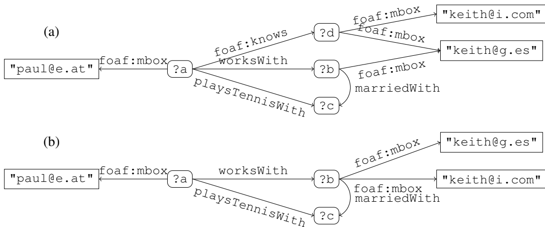
Figure 2.7: RDF graphs.
